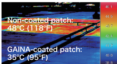
▲The temperature measured in the non-coated patch was 48°C (118°F) and in the GAINA-coated patch, 35°C (95°F).
