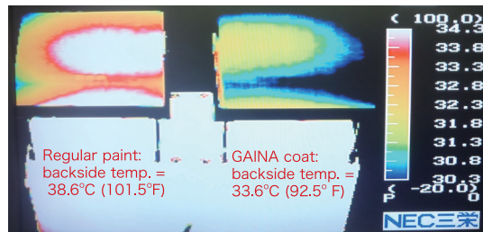
◀The backside temperature of the block with regular paint was 38.6°C (101.5°F), and with GAINA, 33.6°C (92.5°F).
