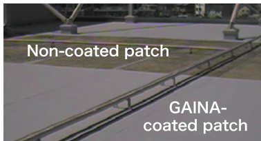
▲Comparison of GAINA-coated and non-coated patches on RC structure roof Test date: September 3, 2008 External temp: 33°C (91°F)
